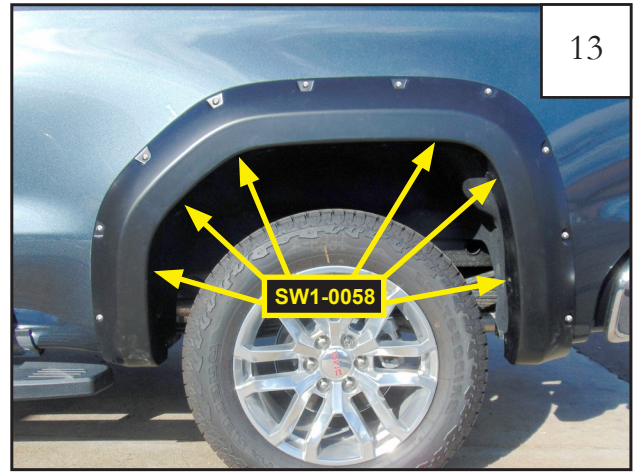
Install rear flare using (6) SW1-0058 truss screws and the (2) outboard screws removed in Step 6.
