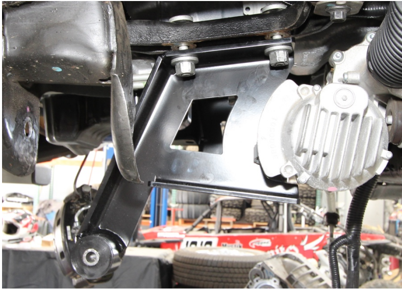
Figure 10: install passenger diff mount
