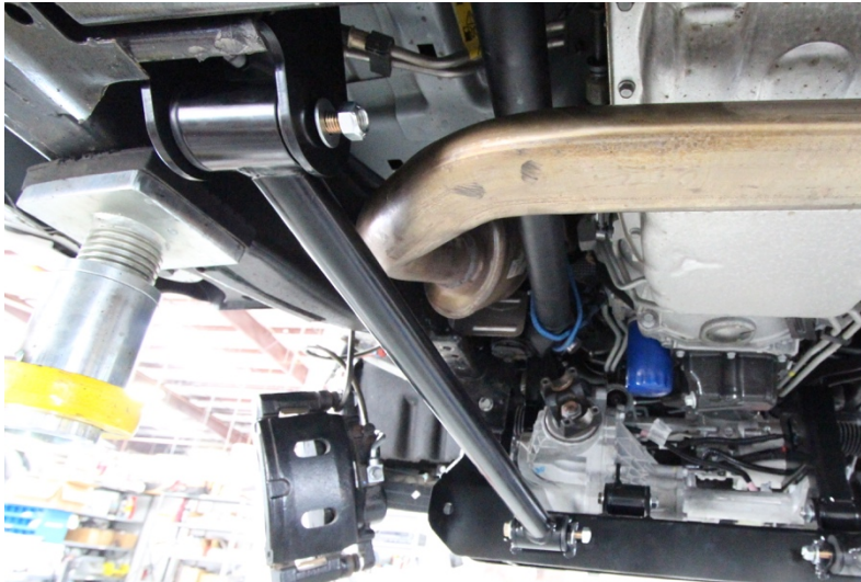
Figure 20: install 8402 compression struts
