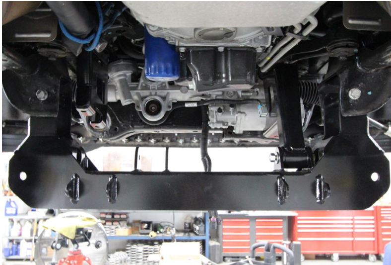
Figure 12: bolt in rear crossmember.
