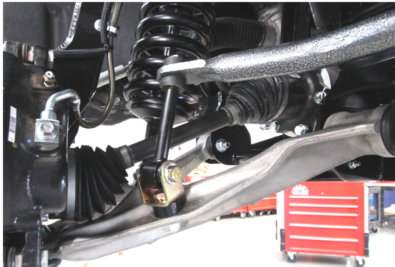
Figure 26: installation of CV axles, sway bar end links with spacers, and brake lines
