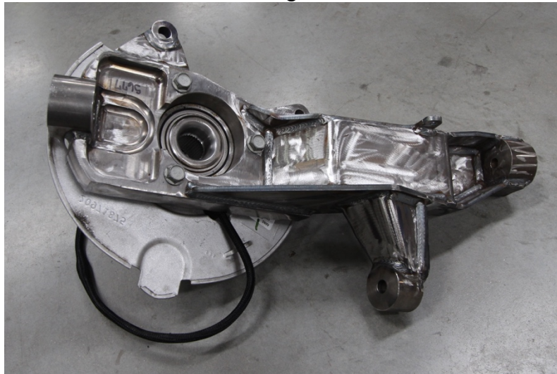
Figure 25: hub transferred to Cognito spindle
