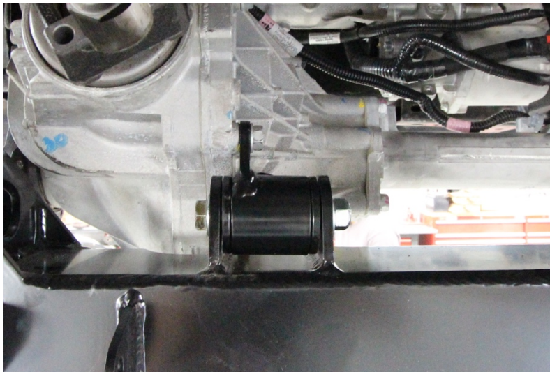
Figure 13: lower diff mount bolted to rear crossmember
