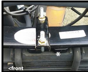
Typical PSP Mounting Kit Installation
